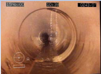
Infiltration Runner- QL install prior to lining
